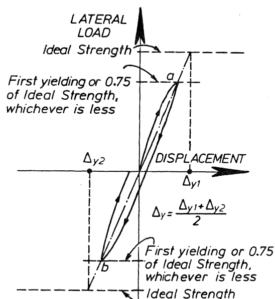
Fig.7 DEFINITION OF YIELD DISPLACEMENT
